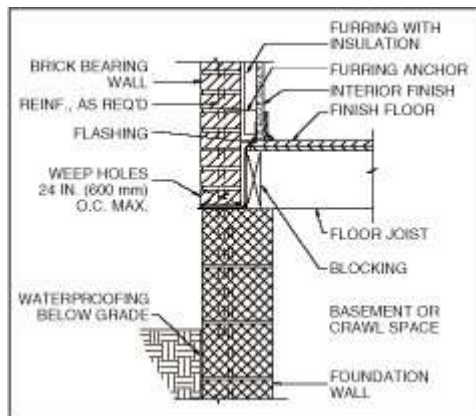
Basement or Crawl Space Foundation Fig. 5
