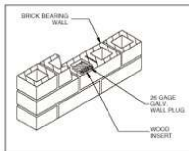
Wall Plug Nailing Insert Fig. 14
