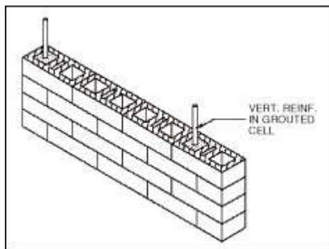
Reinforced Hollow Brick Fig. 3
