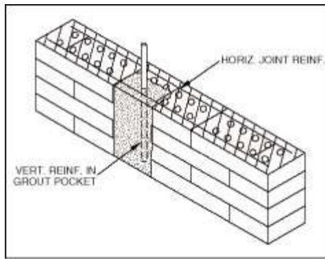
Solid Brick With Grout Pocket Fig. 1
