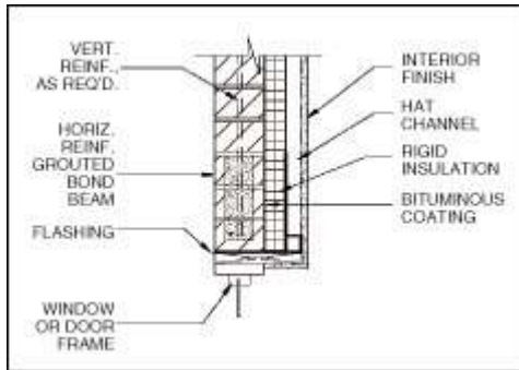
Brick Bond Beam Lintel Fig. 12b
