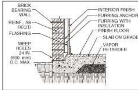
Slab-On-Grade Foundation Fig. 4
