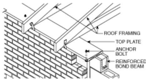
Wood Roof Framing Detail
