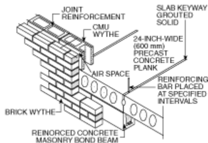
Steel reinforced Concrete Plank Bearing
