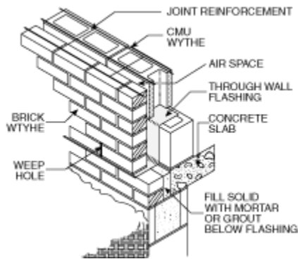
Basement Detail
