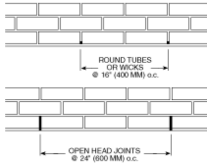
Spacing of Weep Holes
