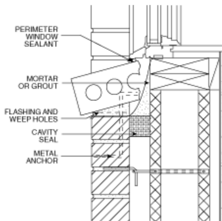
Window Sill Detail
