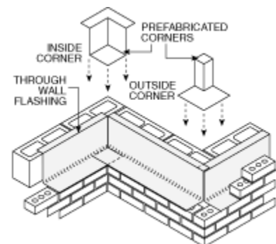
Prefabricated Corners (From Masonry Design and Detailing: For Architects, Engineers, and Contractors, 4th Edition, Christine Beall )
