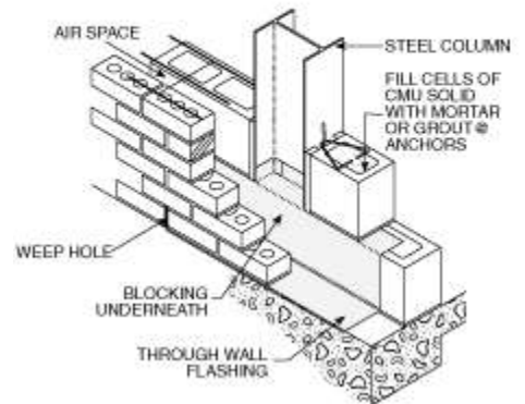
Flashing at Steel Column
