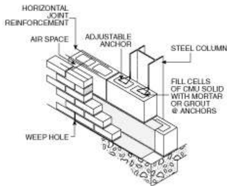
Anchorage to Steel Column
