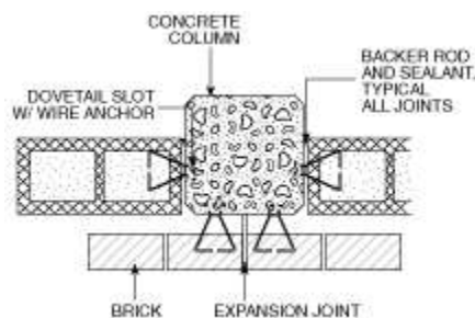
Vertical Expansion Joint
